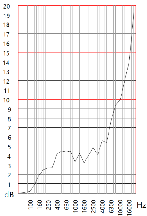
Barrier performance measured in the workplace. Barrier dimensions: 1300xH2500mm. Measurement performed at 1m distance
